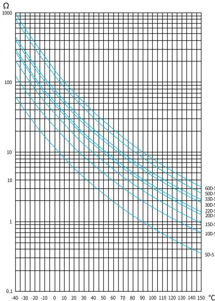
温度特性曲线 Resistance-Temperature Characteristic
