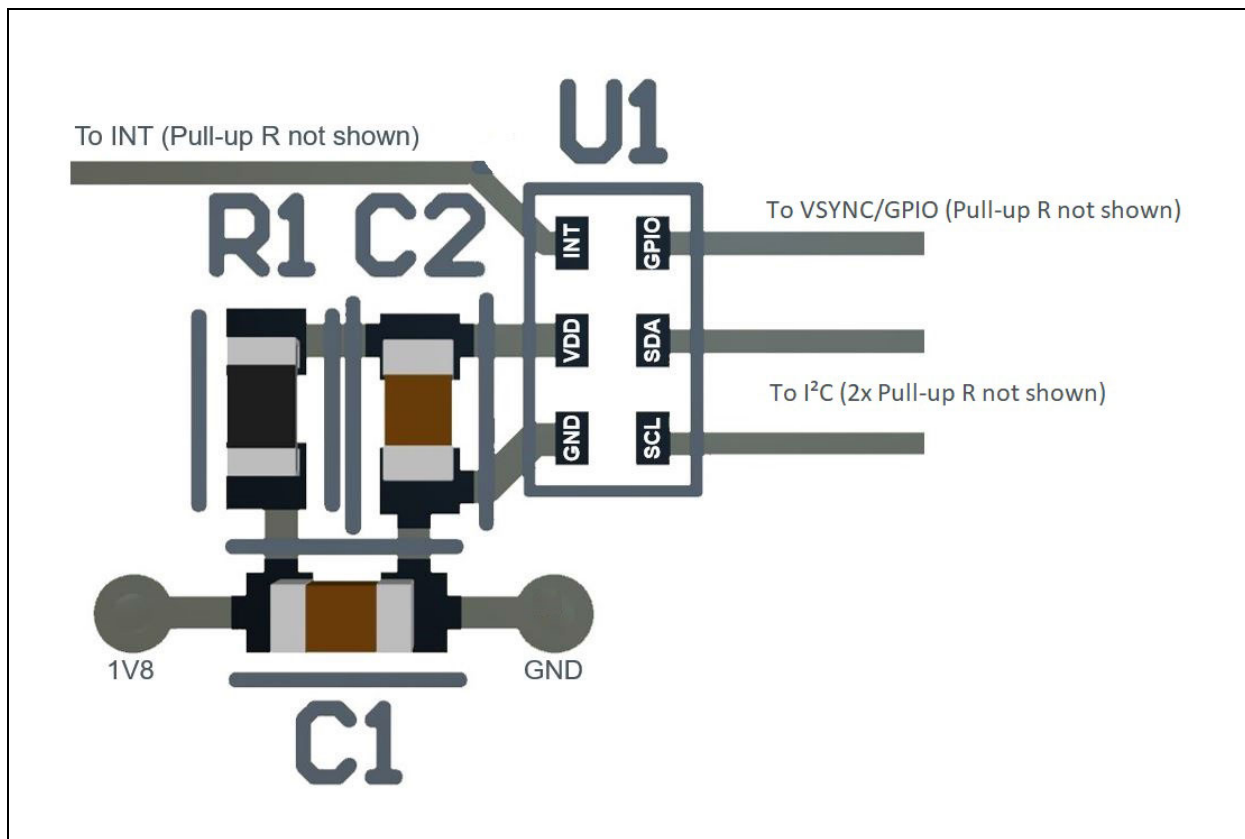
Figure 93: TCS3410 Recommended Part Placement
