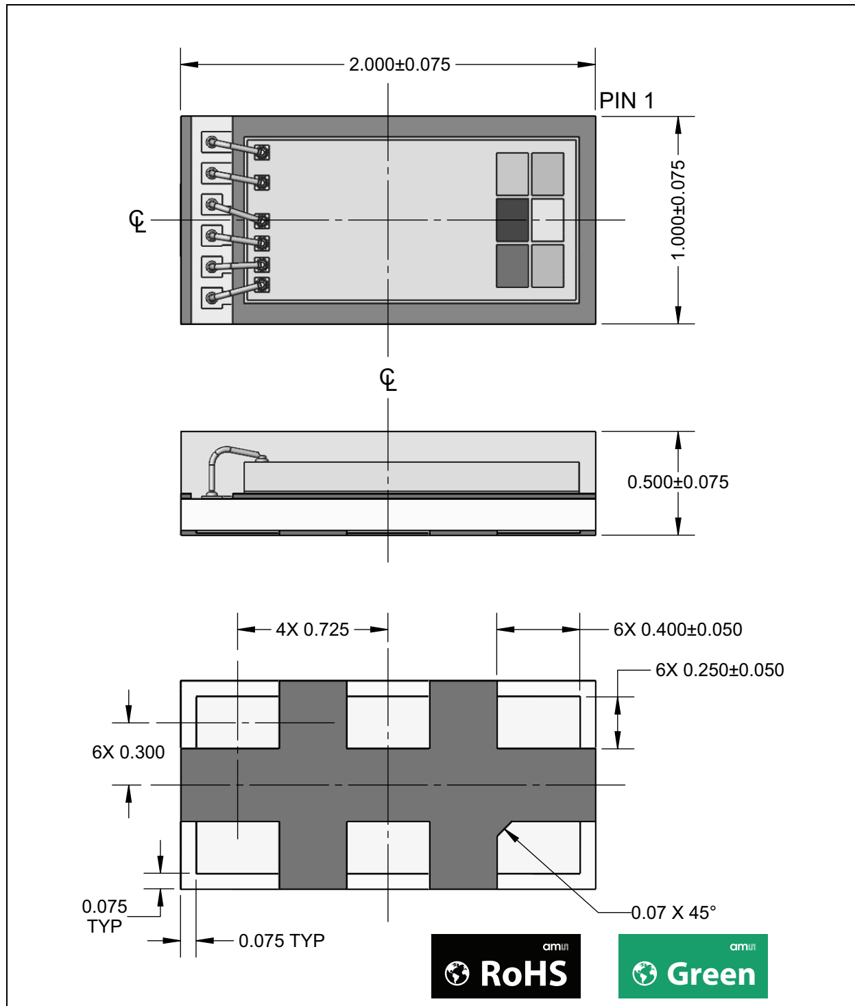
Figure 94: TCS3410 Module Dimensions
