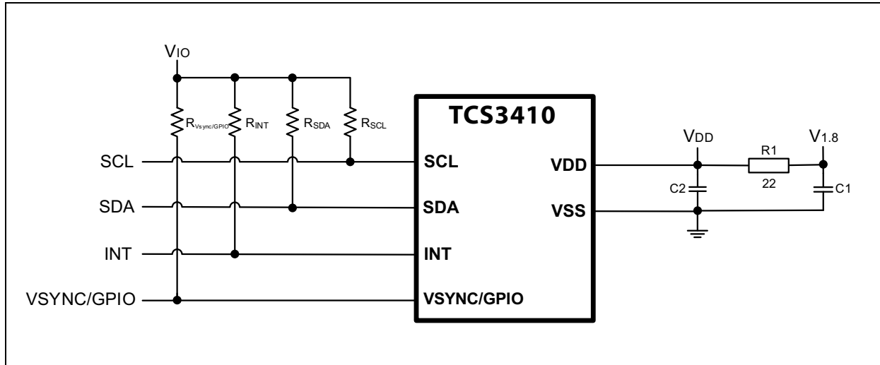
Figure 92: TCS3410 Typical Application Circuit
