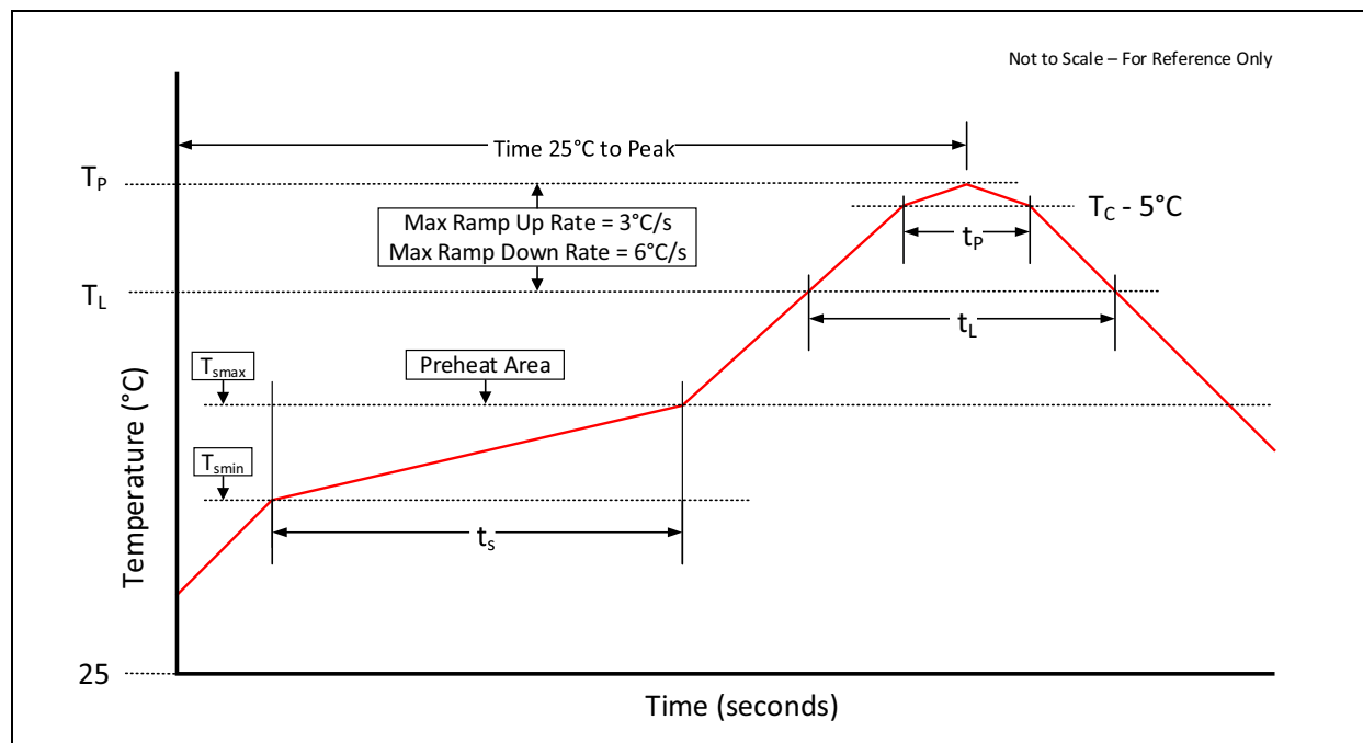
Figure 98: Solder Reflow Profile Graph
