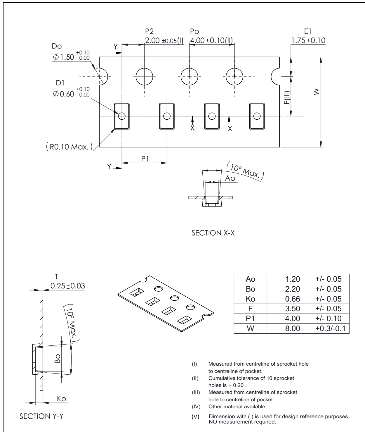
Figure 96: Tape and Reel Mechanical Drawing
