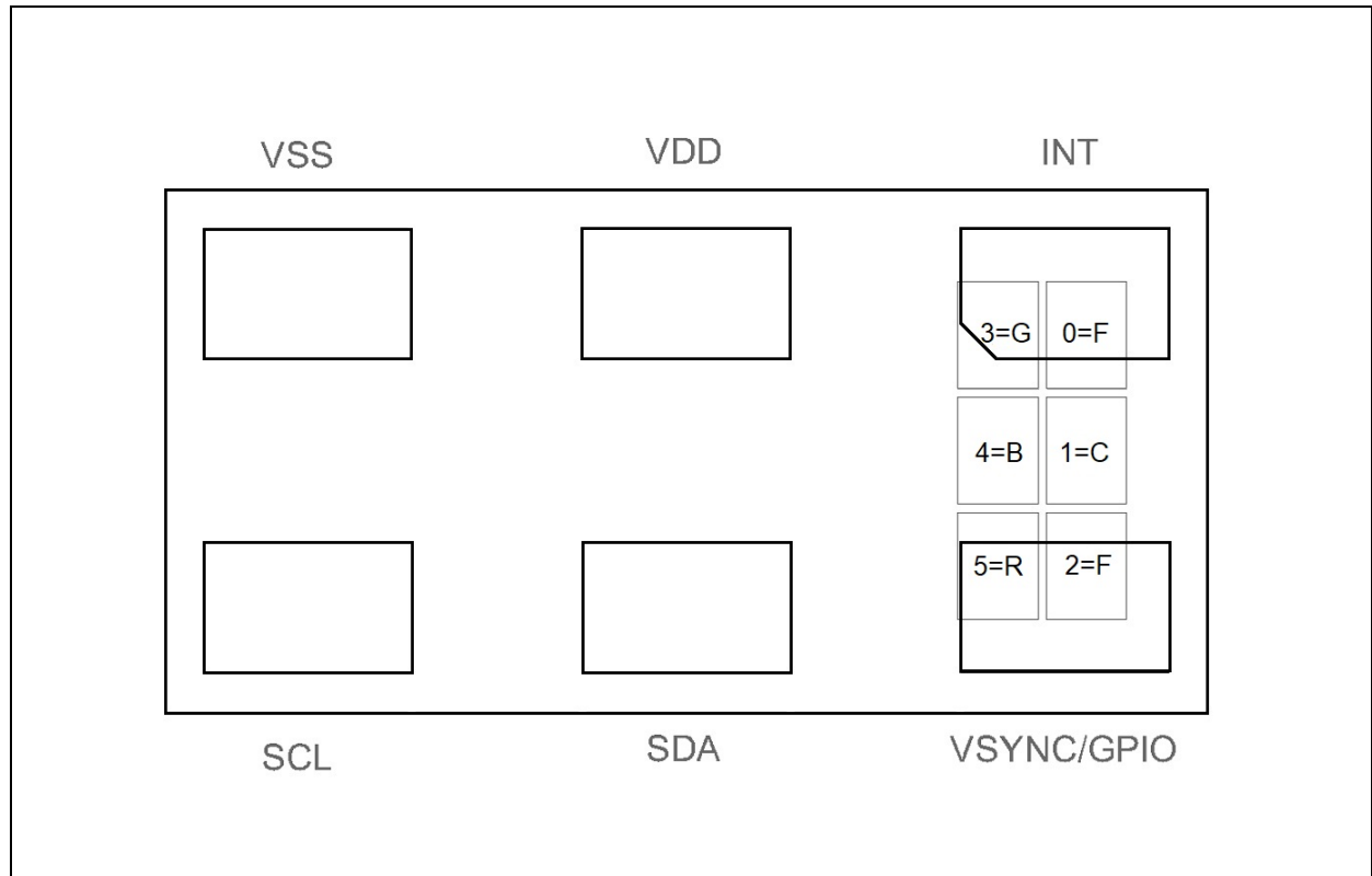
Figure 3: Pin Diagram and Photodiode Location of TCS3410 (top view)
